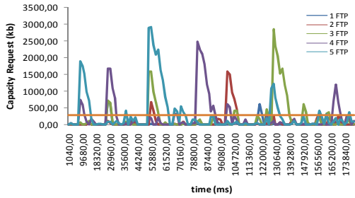
Figure 5. FTP capacity request for a small number of users.
