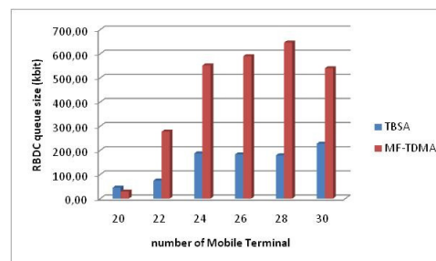
Figure 10. RBDC queue size comparison between classical MF-TDMA system and a system with a 90% of MF-TDMA and 10% of SCPC and the TBSA algorithm.
