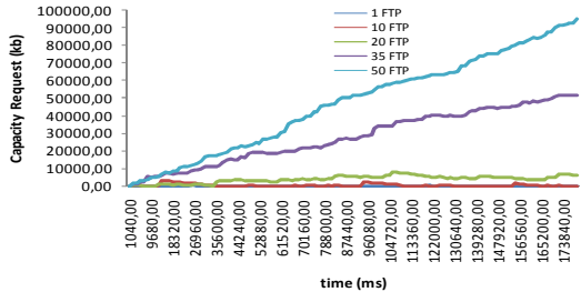
Figure 6. FTP capacity request for a great number of users.
