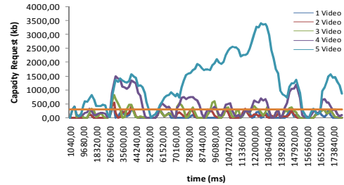
Figure 8. Video Conference capacity request for a small number of users.
