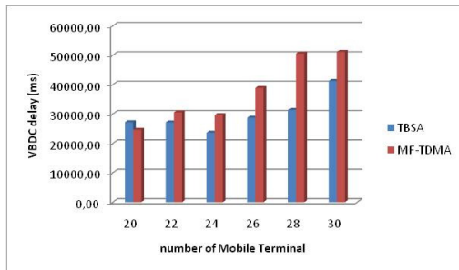
Figure 13. VBDC delay comparison between classical MF-TDMA system and a system with a 90% of MF-TDMA and 10% of SCPC and the TBSA algorithm.
