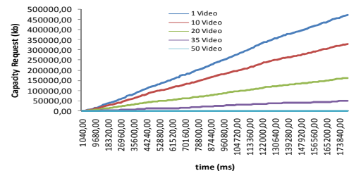
Figure 9. Video Conference capacity request for a great number of users.
