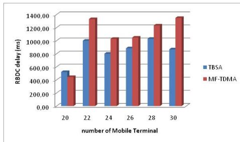
Figure 12. RBDC delay comparison between classical MF-TDMA system and a system with a 90% of MF-TDMA and 10% of SCPC and the TBSA algorithm.
