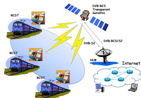
Figure 1. DVB-RCS+M Architecture.
